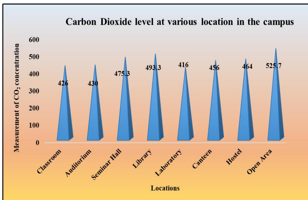
Figure 5. Measurement of CO 2 concentration in the Campus
