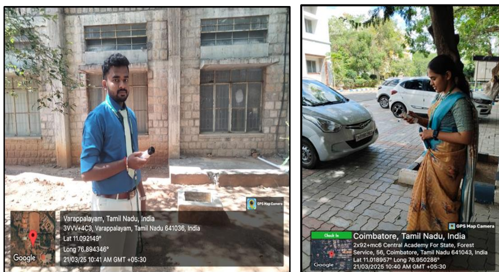
Measurement of O 2 level at the Campus
