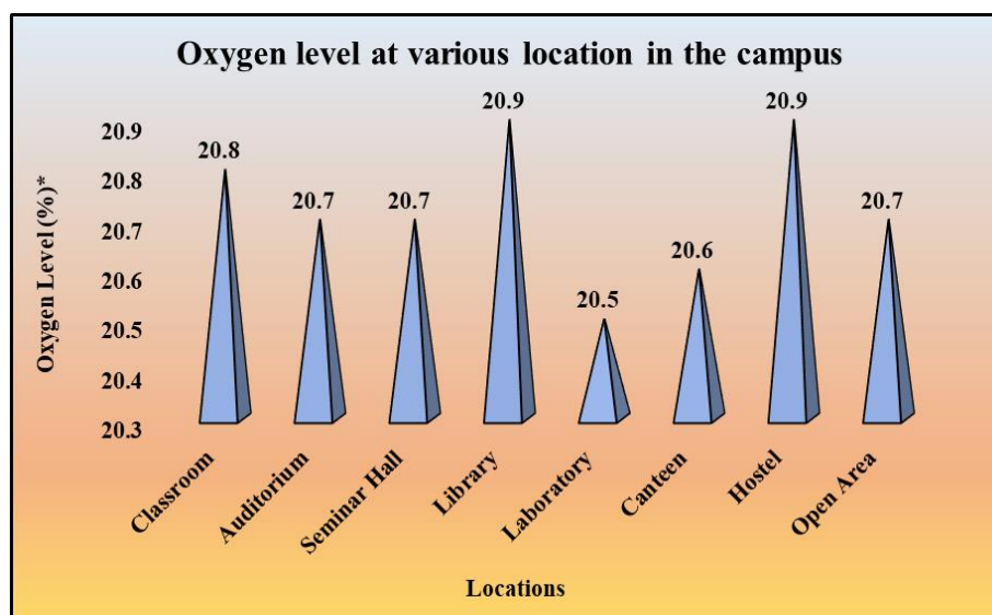
Figure 6. The oxygen concentration in the Campus
