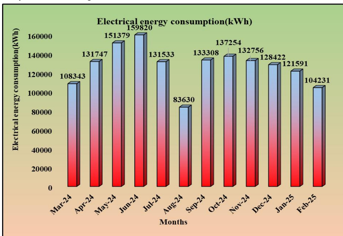
Figure 1. Electrical energy consumption profile
